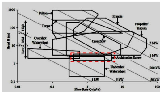
Fig. 1. Classification of Thread Turbine's with Head and Output Power
