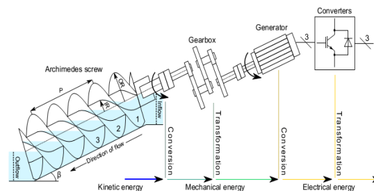
Fig. 2. Turbine Schematic of Archimedes Screw
